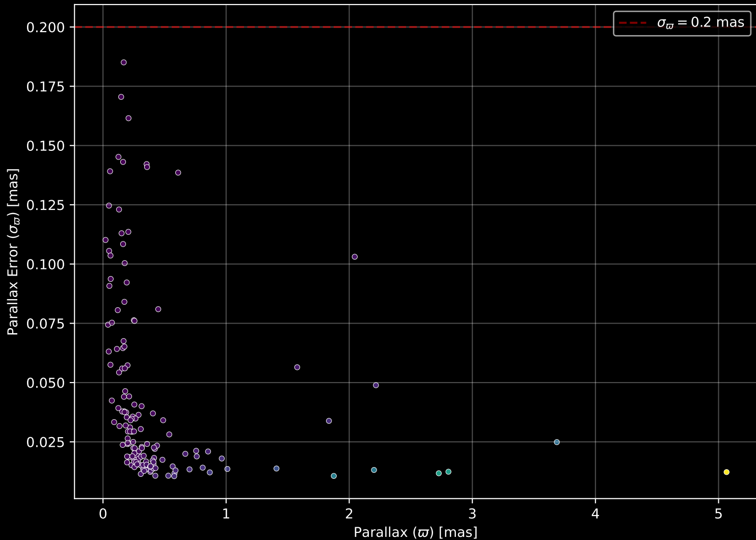
APOGEE DR17 Field: [285+00] Parallax Quality (n= 148)
