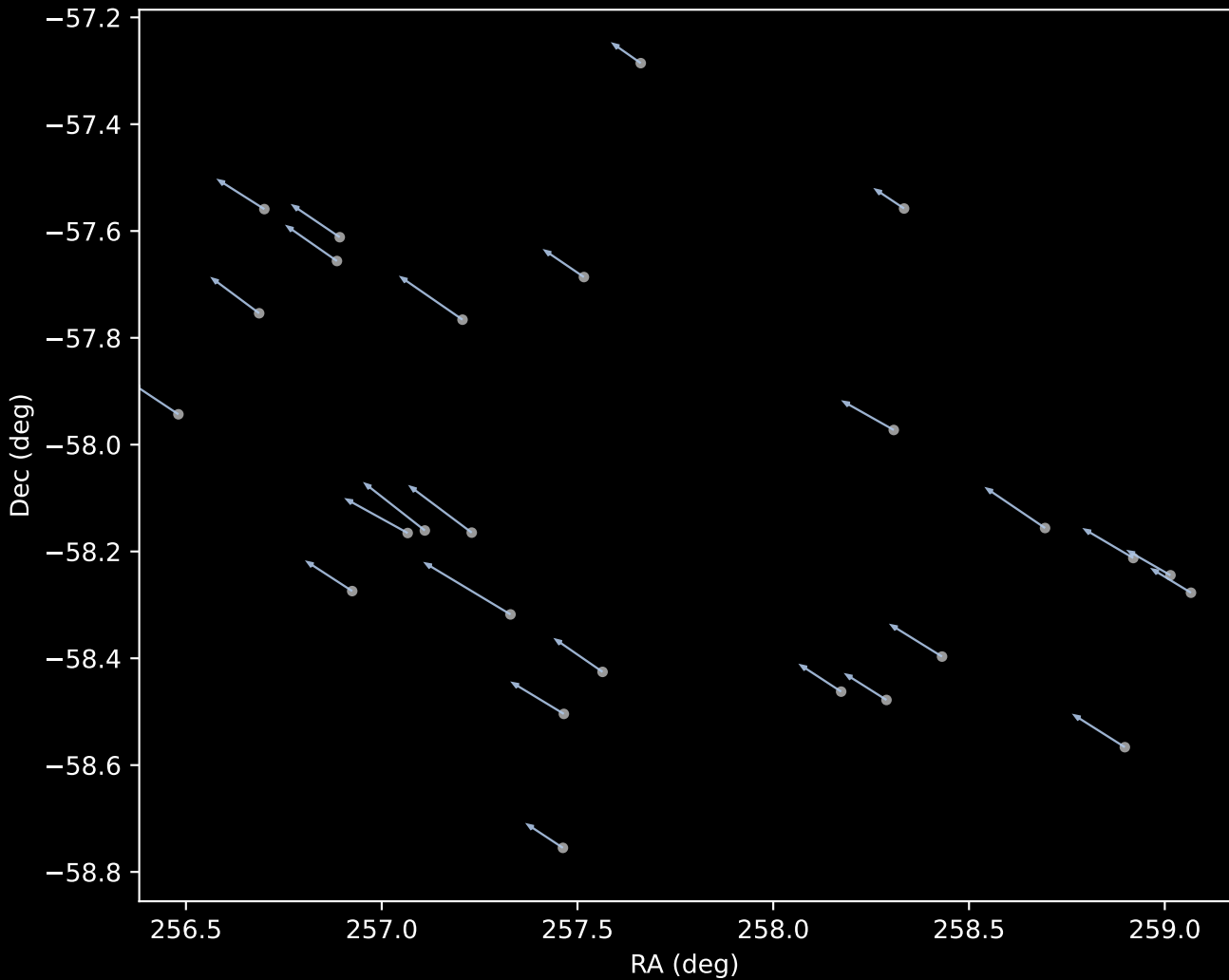
APOGEE DR17 Cluster 1 Proper Motion Vectors (n=26)
