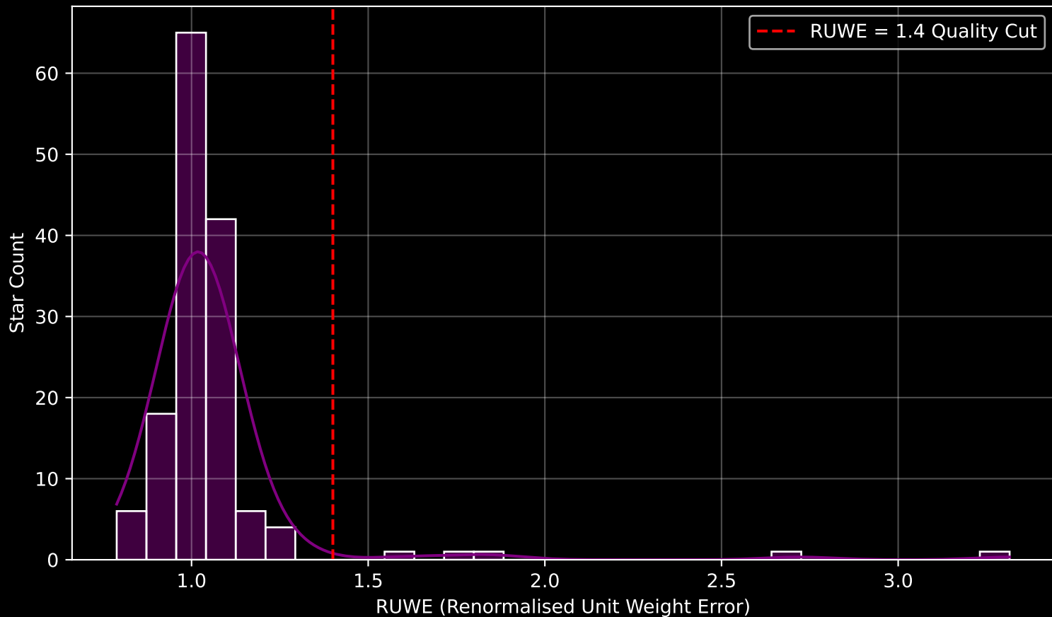
GAPOGEE DR17 Field [285+00] RUWE Distribution (n= 146)
