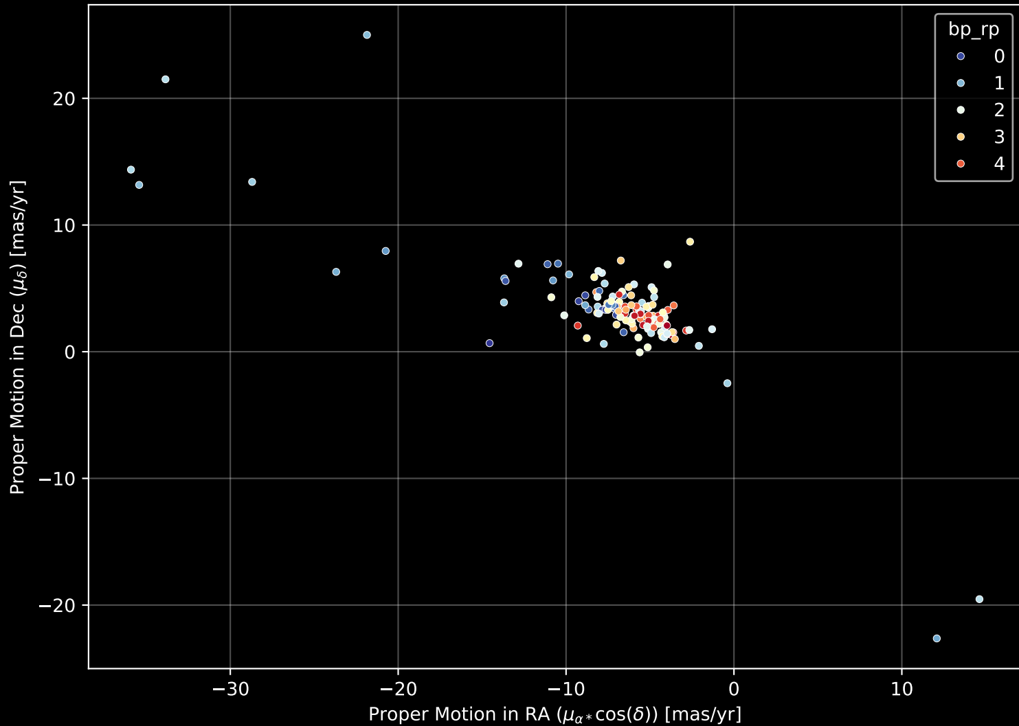
APOGEE DR17 Field: [285+00] Proper Motion Diagram (n= 148)
