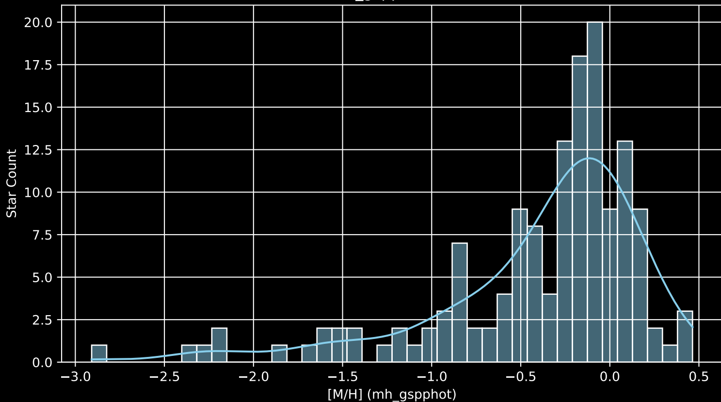
APOGEE DR17 Field: [285+00 [M/H] (mh_gspphot) (n= 146)
