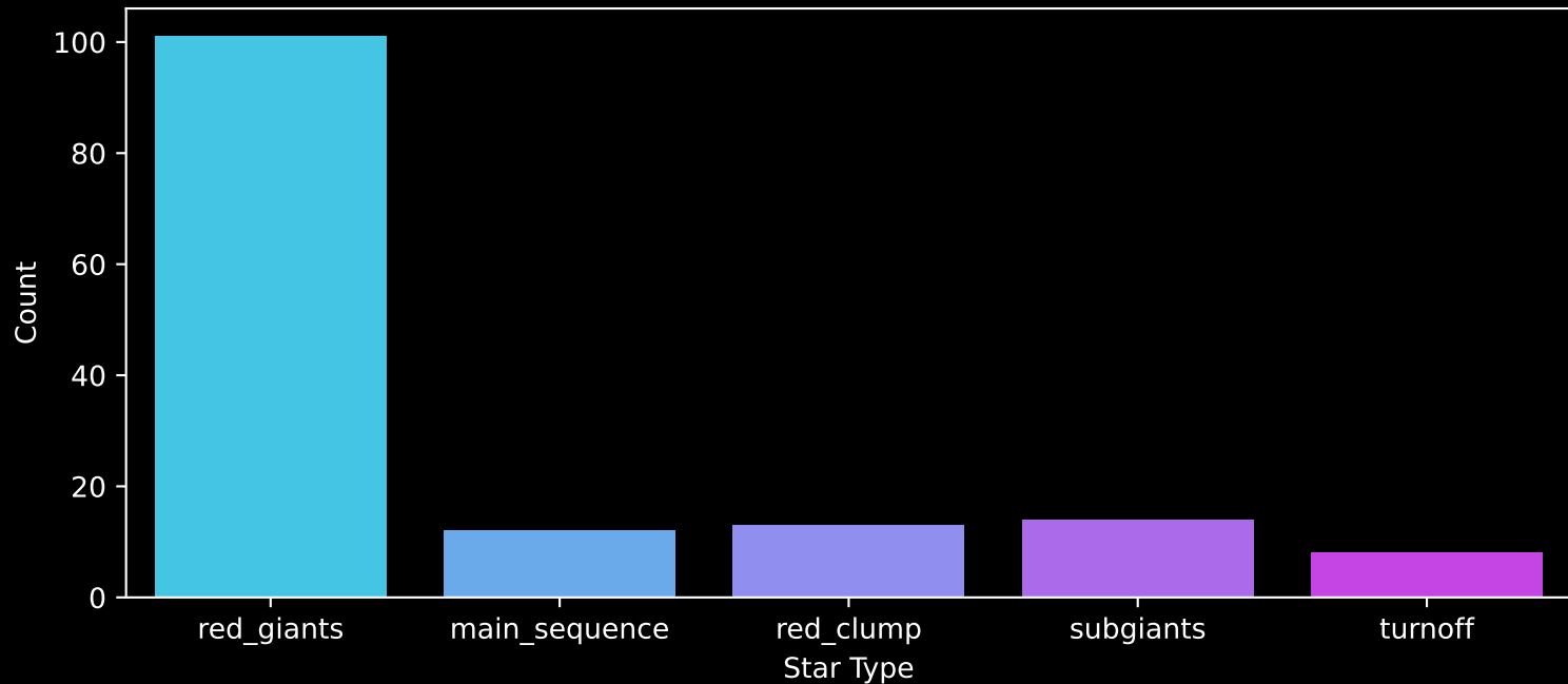
APOGEE DR17 Field: [285+00] Count plot of Star Type
